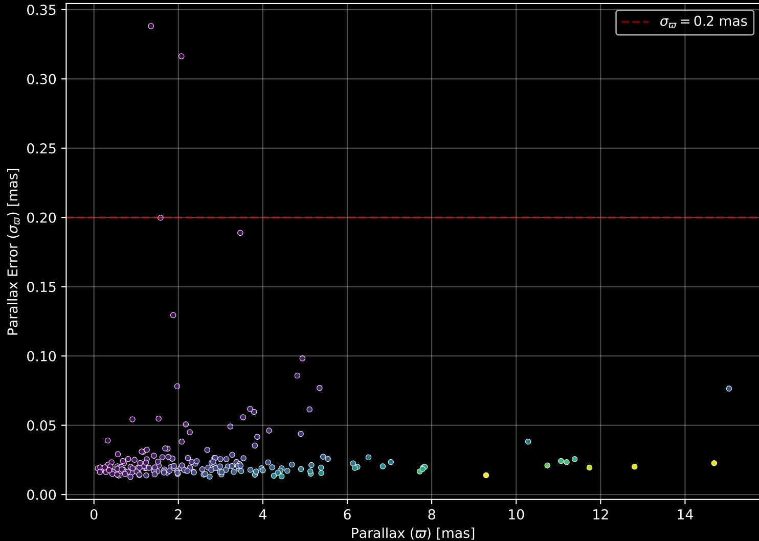
APOGEE DR17 Field: [237+38_MGA] Parallax Quality (n= 187)
