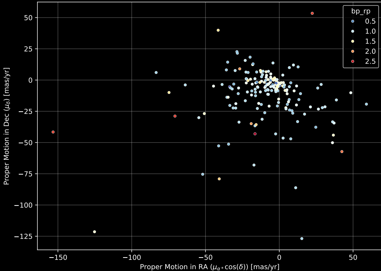
APOGEE DR17 Field: [237+38_MGA] Proper Motion Diagram (n= 187)
