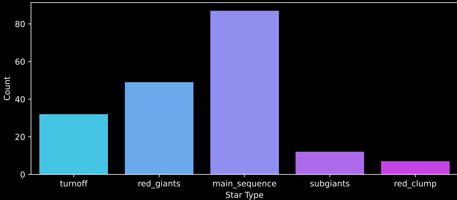
APOGEE DR17 Field: [237+38_MGA] Count plot of Star Type
