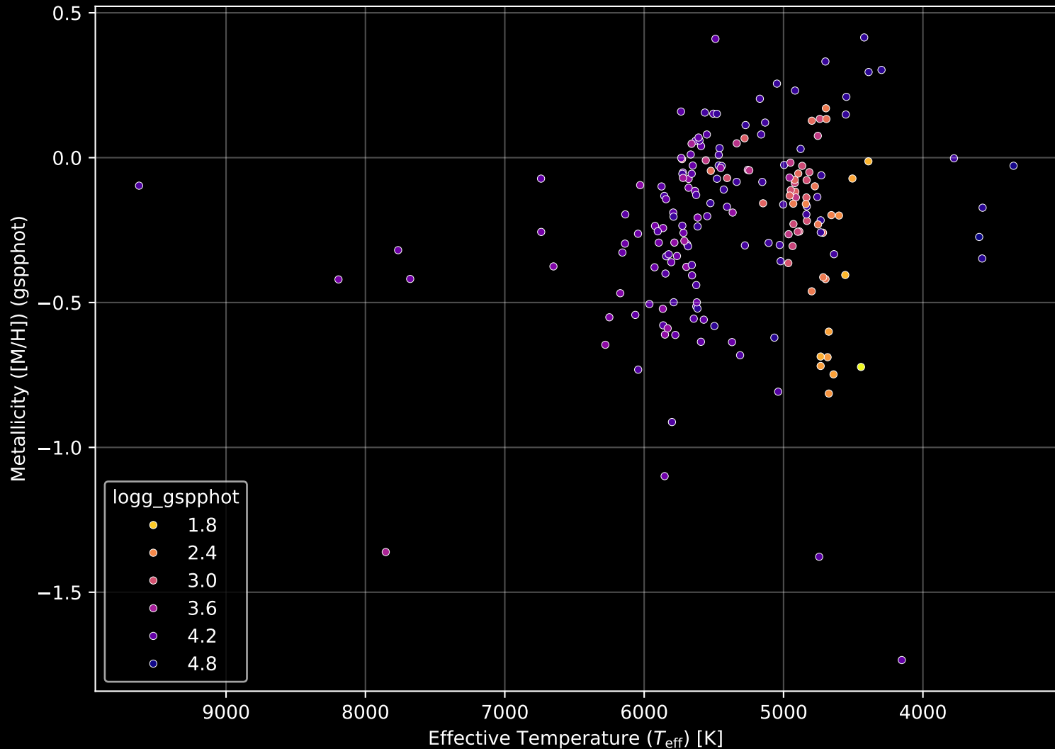
APOGEE DR17 Field: [237+38_MGA] Stellar Population Parameters (n= 187)
