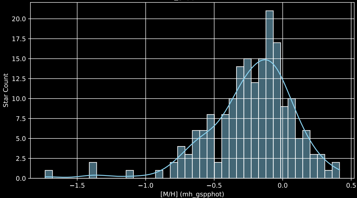
APOGEE DR17 Field: [237+38_MGA [M/H] (mh_gspphot) (n= 187)
