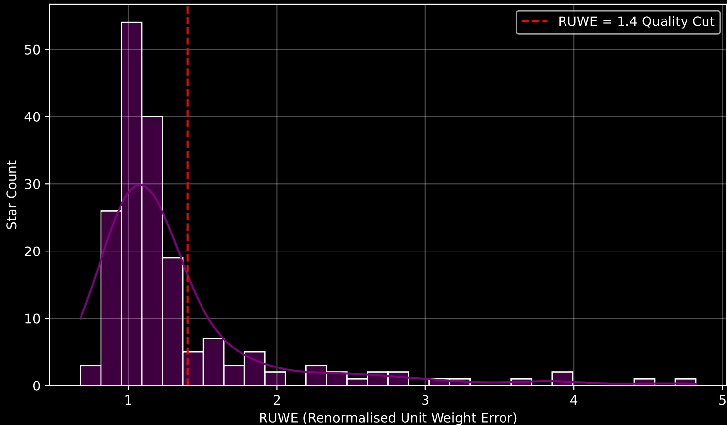
GAPOGEE DR17 Field [237+38_MGA] RUWE Distribution (n= 181)
