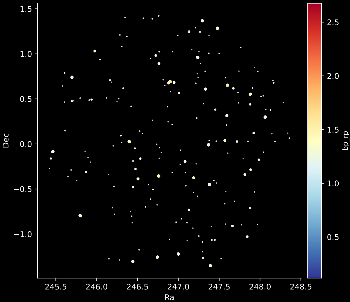
APOGEE DR17 Field: [237+38_MGA] Stars: 187
